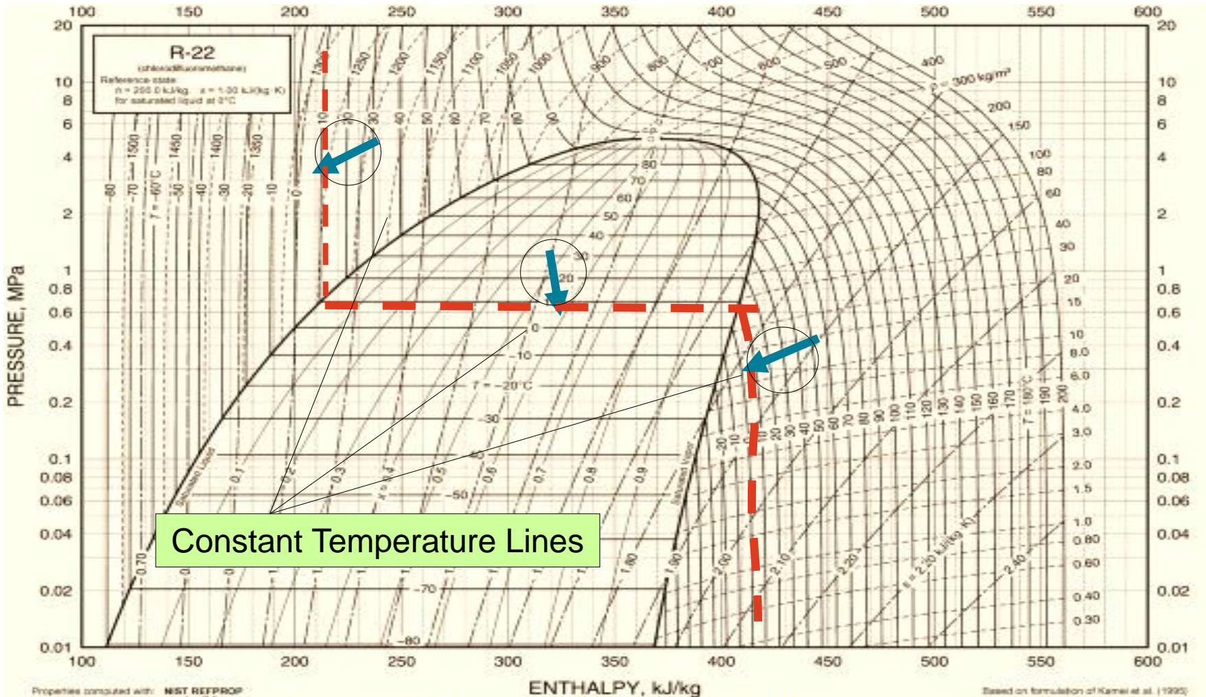
Fig. 2 Pressure-Enthalpy Diagram for Refrigerant 22
